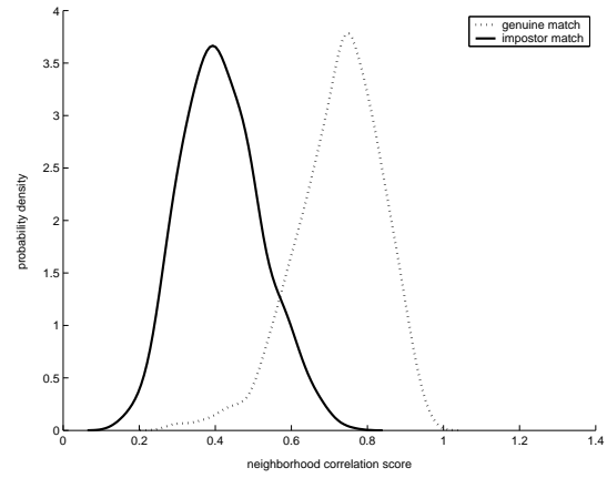
Fig. 6. Histograms of neighborhood correlation scores of DB1.
