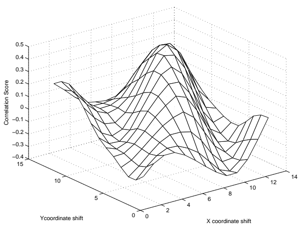
Fig. 2. Local maximum correlation searching for neighborhood alignment.
