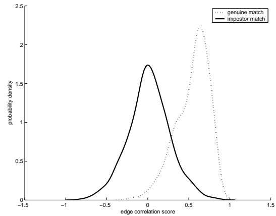
Fig. 7. Histograms of edge correlation scores of DB1.
