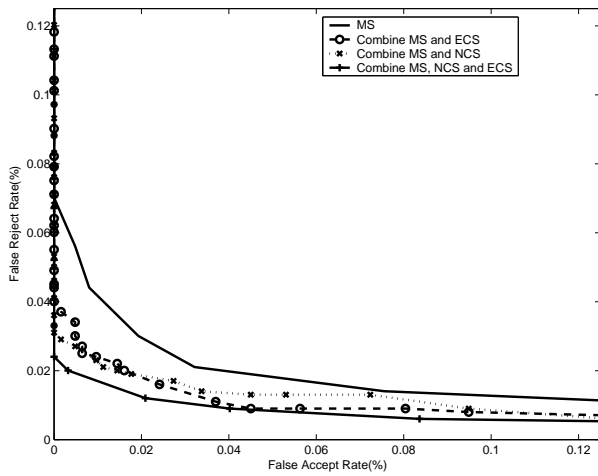
Fig. 8. ROC curves of different score combinations of DB1 data set. MS: Minutiae score. NCS: Neighborhood correlation score. ECS: Edge correlation score. Combining rule: product rule.
